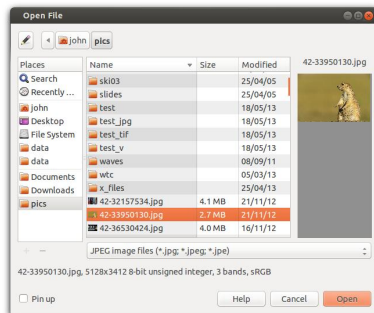
Figure 4.4: Open dialog
